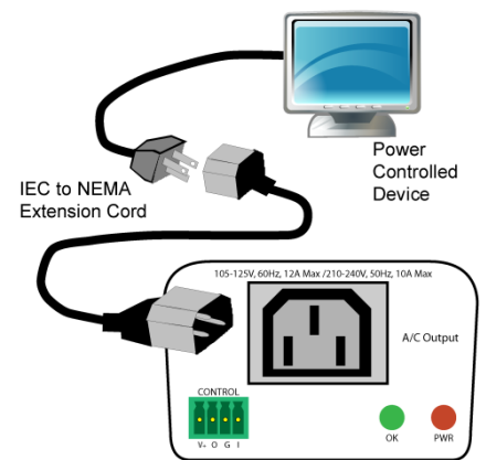
Connect Powered Device using Supplied Cord
