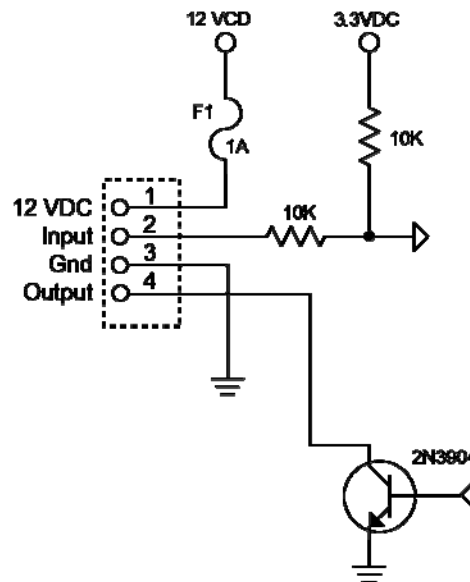
Electrical Connections for Control and Feedback
